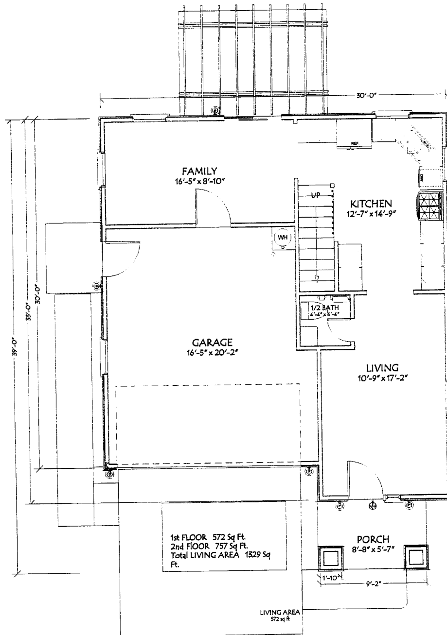
30x39' The Sacramento Country Modern 1st Floor Plan.
