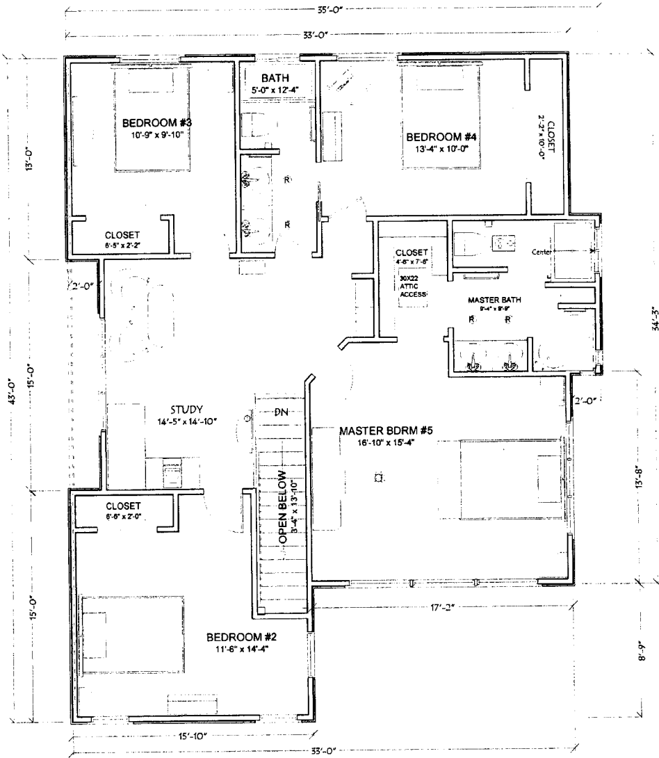
The MidWesterner 35x54' 2nd Floor Plan.
