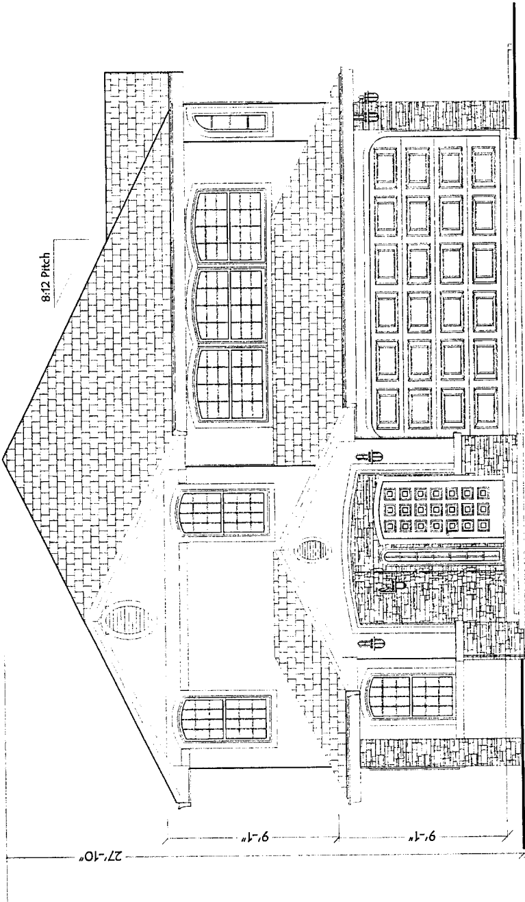
The MidWesterner 35x54' Optn.-A Front Elevation.
