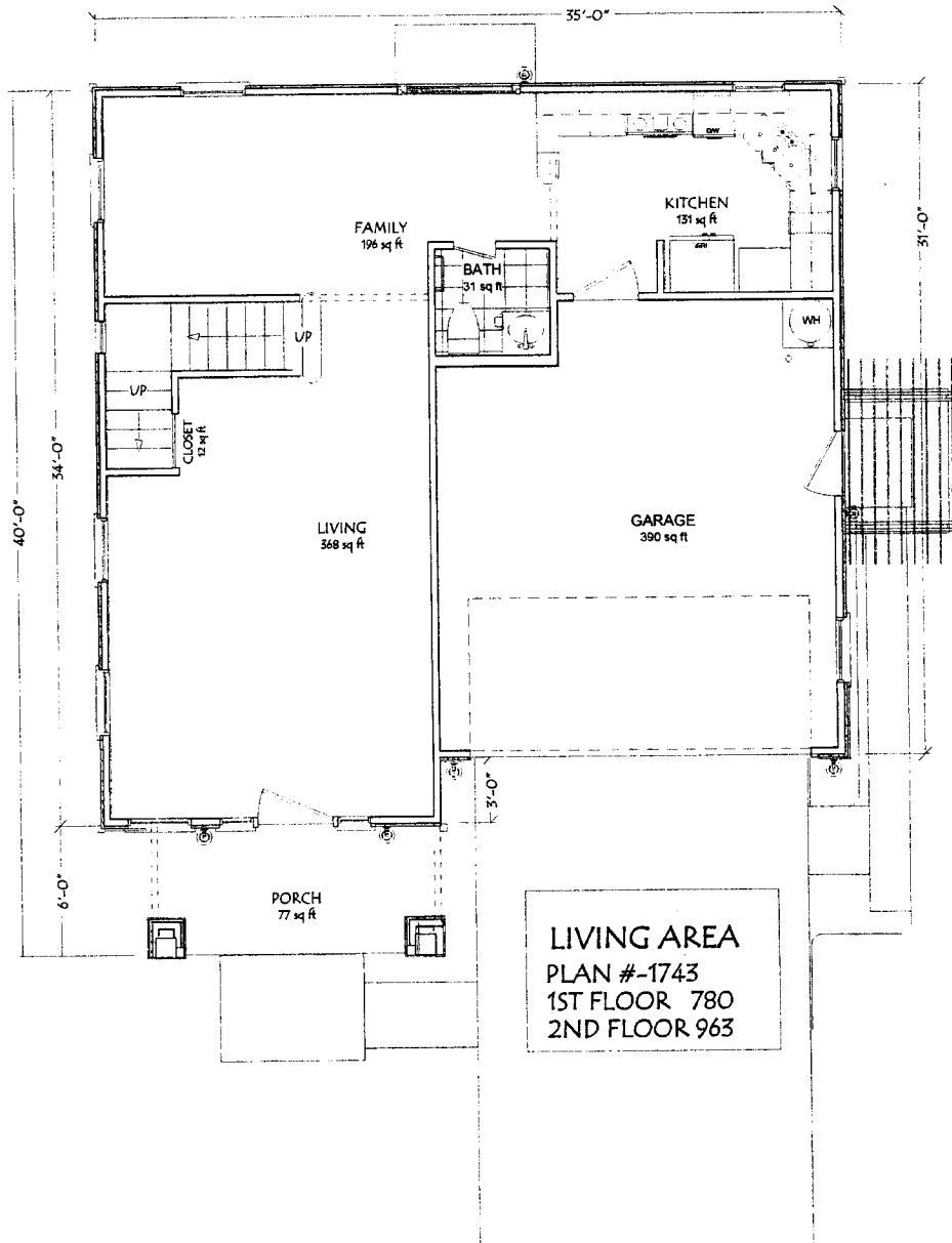
The New Orleans 35x40' 1st Floor Plan.
