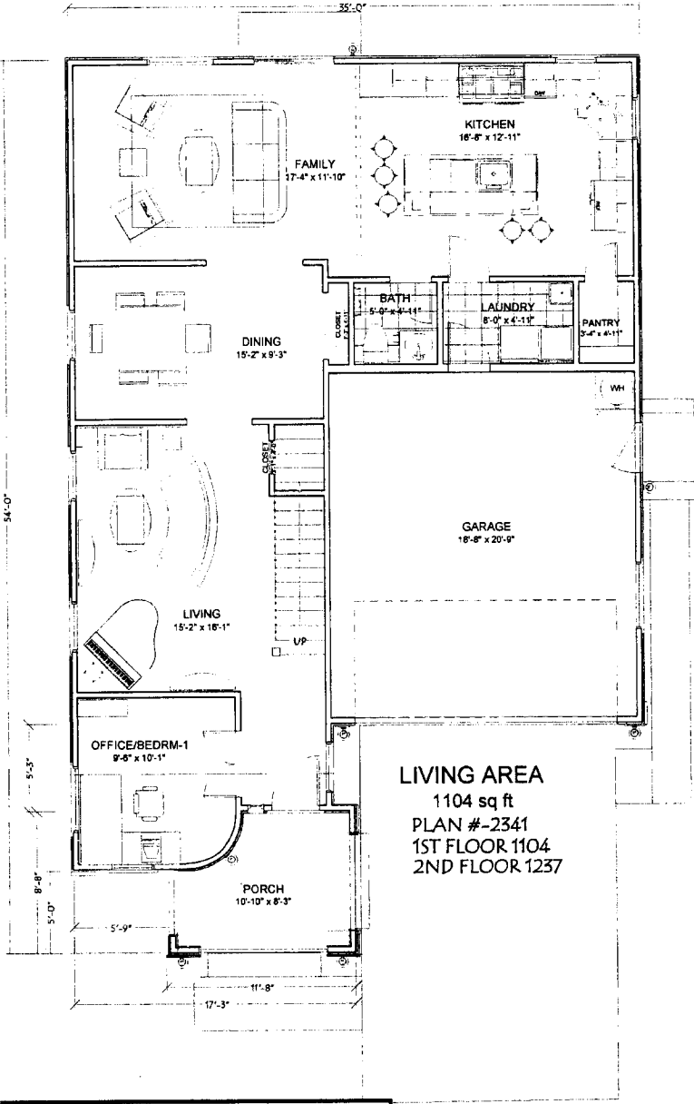
The MidWesterner 35x54'
