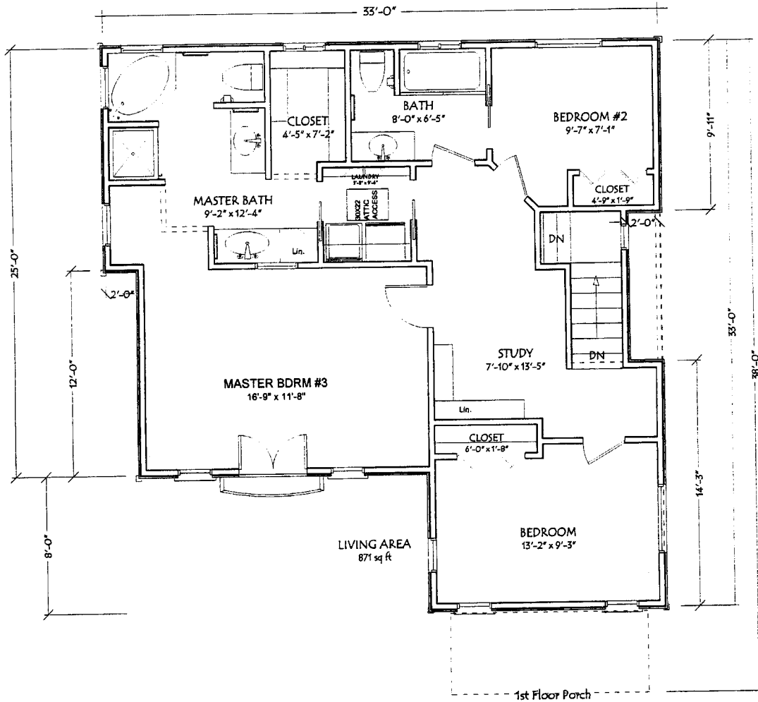
The Sacramento Country Modern Optn.-A 2nd Floor Plan.
