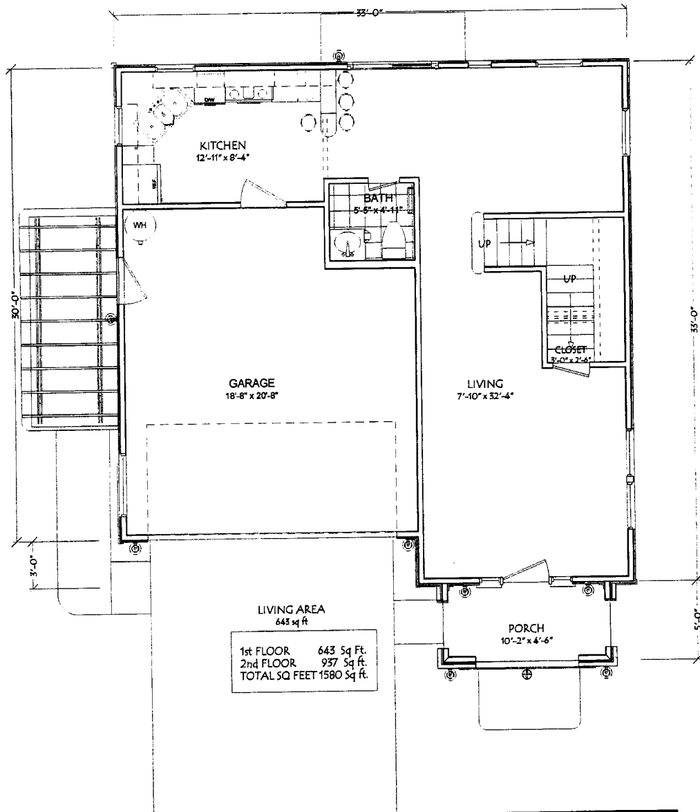
The Sacramento Country Modern Optn.-A 1st Floor Plan.
