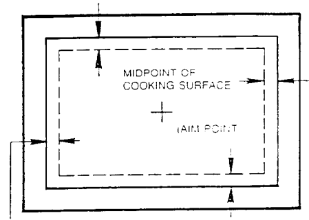
260 NOZZLE LOCATED ALONG ANY SIDE OF GRIDDLE SURFACE WITHIN 0 - 2 IN. (0 - 5.1 CM) OF COOKING SURFACE EDGE. NOZZLE MUST BE AIMED AT MIDPOINT OF COOKING SURFACE.
