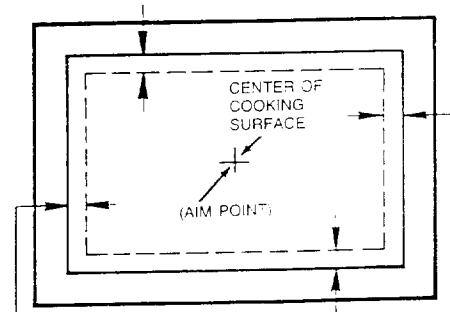
290 NOZZLE LOCATED ALONG ANY SIDE OF GRIDDLE SURFACE WITHIN 0 - 2 IN. (0 - 5.1 CM) OF COOKING SURFACE EDGE. NOZZLE MUST BE AIMED AT CENTER OF COOKING SURFACE.
