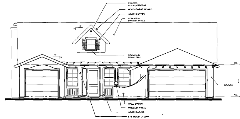
PLAN 652 - MONTEREY FRONT ELEVATION A
