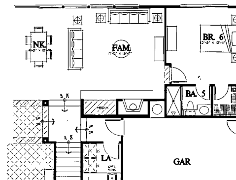
PLAN 654 - OPTION 4 BEDROOM OPTION 248 SQ. FT.
