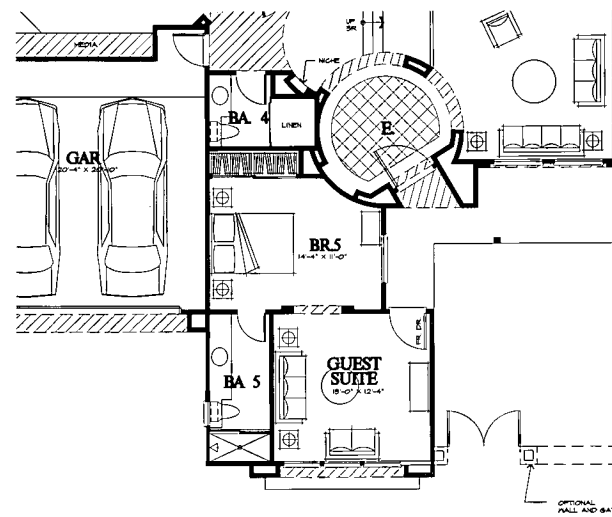
PLAN 655 - OPTION 2 GUEST SUITE OPTION 240 SQ. FT.
