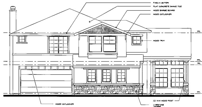
PLAN 655 - CRAFTSMAN FRONT ELEVATION B
