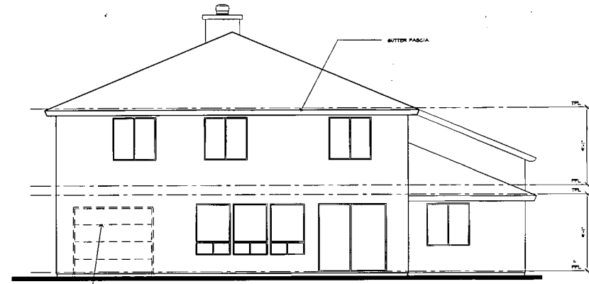
REAR ELEVATION A
