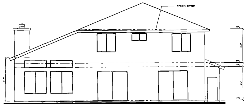
REAR ELEVATION A
