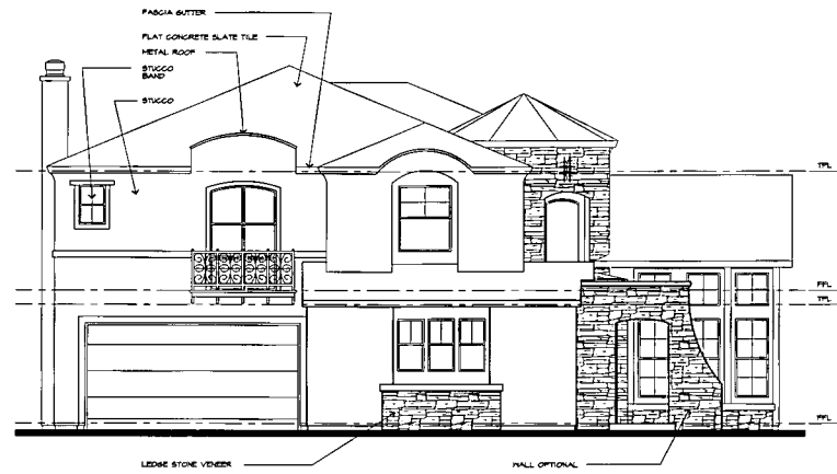
PLAN 655 - FRENCH COUNTRY FRONT ELEVATION B
