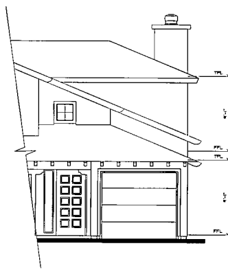
PLAN 653 - MONTEREY FRONT ELEVATION A OPTION 3
