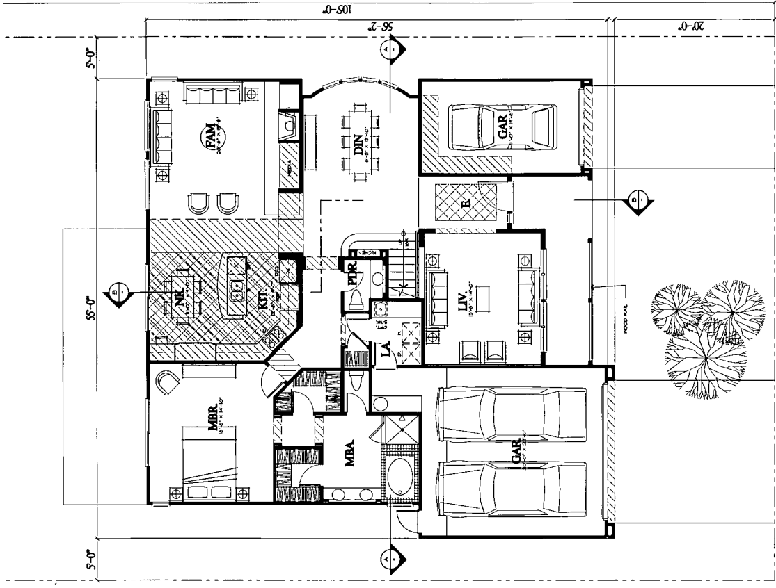
LOWER LEVEL A COURT YARD AREA (NOT TO SCALE)
