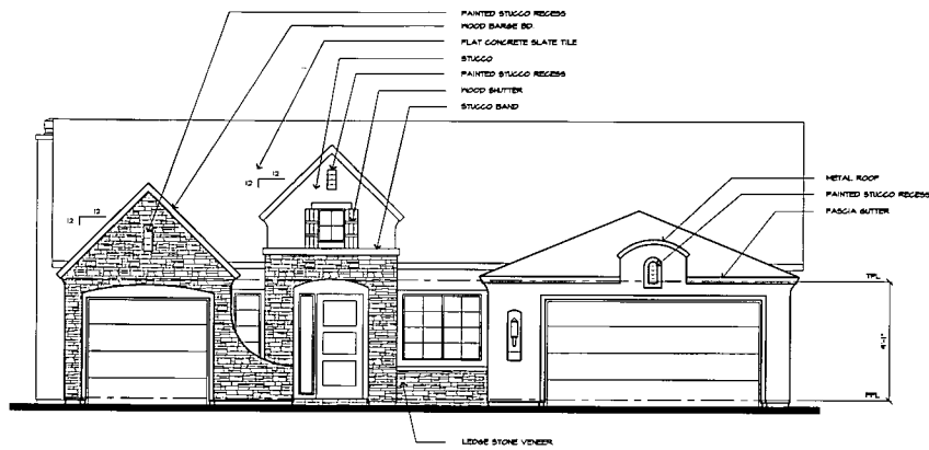
PLAN 652 - FRENCH COUNTRY FRONT ELEVATION C
