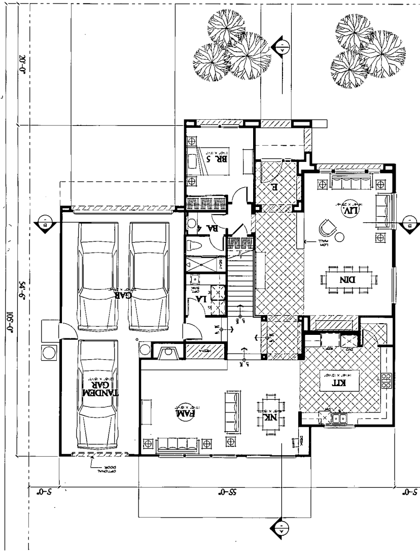
LOWER LEVEL A LOWER FLOOR AREA: 1,789 SQ. FT.
