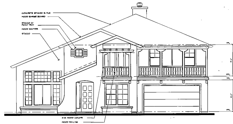
PLAN 654 - MONTEREY FRONT ELEVATION A
