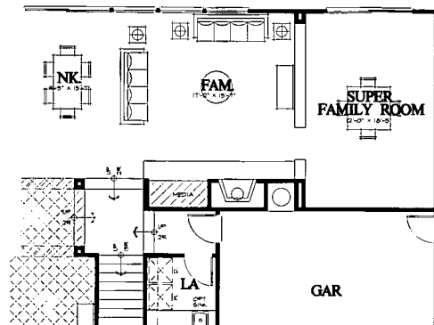
PLAN 654 - OPTION 3 SUPER FAMILY ROOM OPTION 248 SQ. FT.
