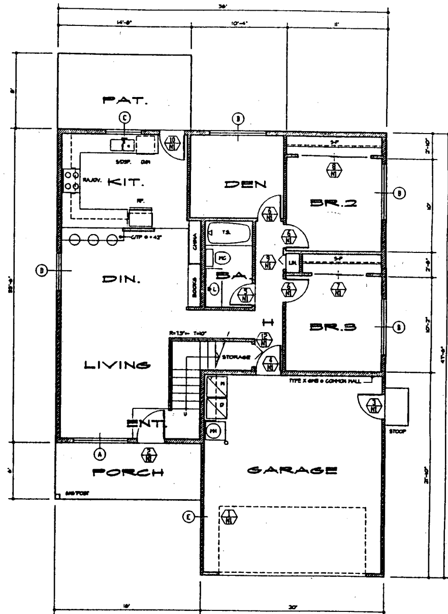
FLOOR PLAN @ FIRST
