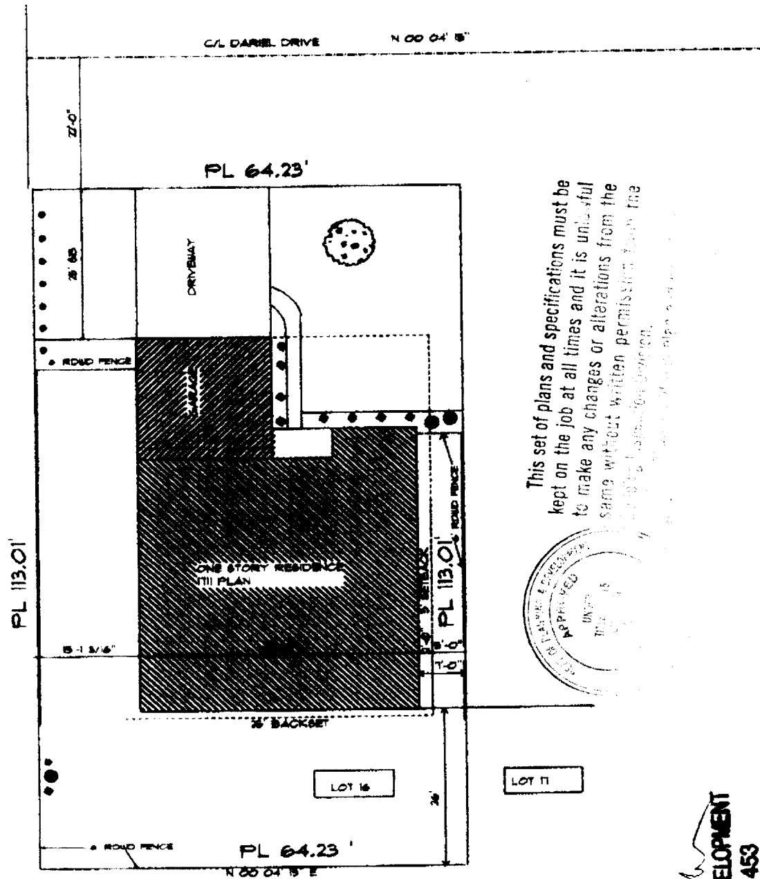
PLOT PLAN LOT 16
