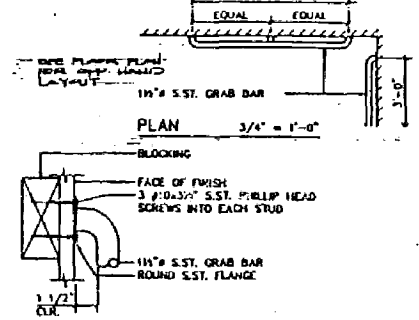
ⓓ TYPICAL GRAB BAR 3'-1'-0"
