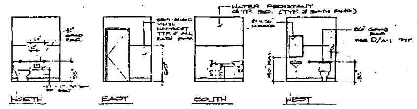
ⓑ P.C. BATH ROOM - INTERIOR ELEVATIONS 1/4" = 1'-0"
