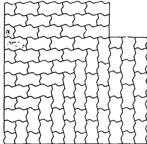
90° directional change
