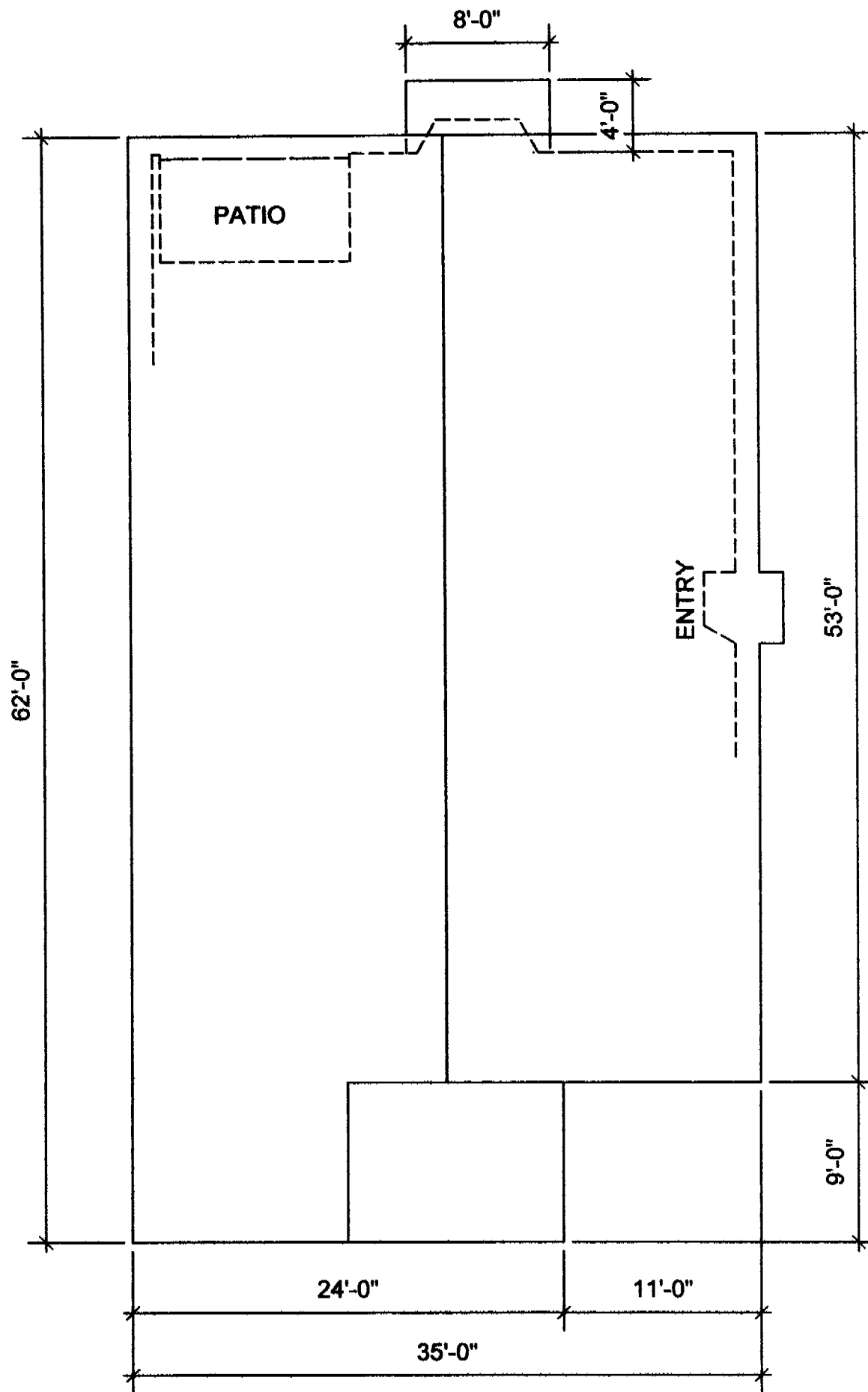
3437 RANCHO RIO WAY SCHEMATIC ROOF PLAN (DIMENSIONS ARE APPROXIMATED)
